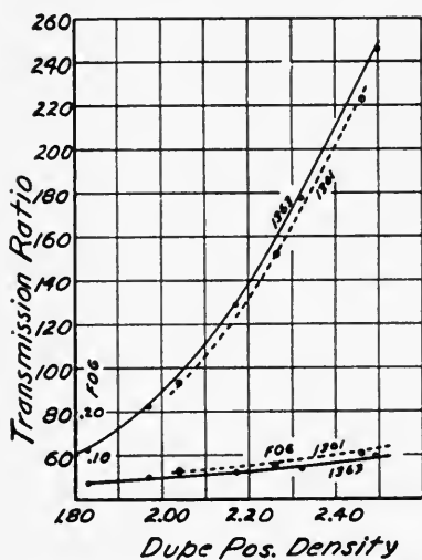
FIG. 3. Transmission ratio chart of 1301 and 1363 stocks as a function of fog.
